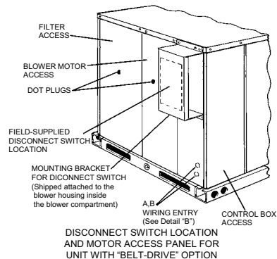
FIGURE 8 - DISCONNECT/BLOWER ACCESS LOCATION
